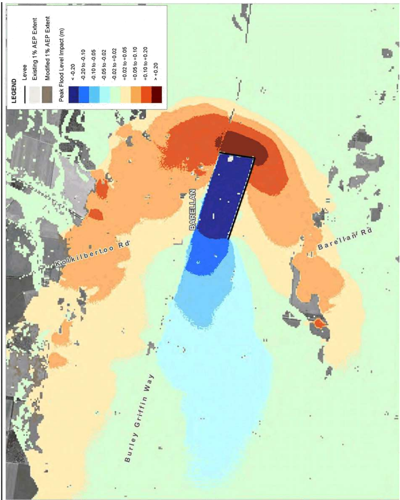
Title: Barellan FRMS&P Levee Option 1d Extreme Flood Event
