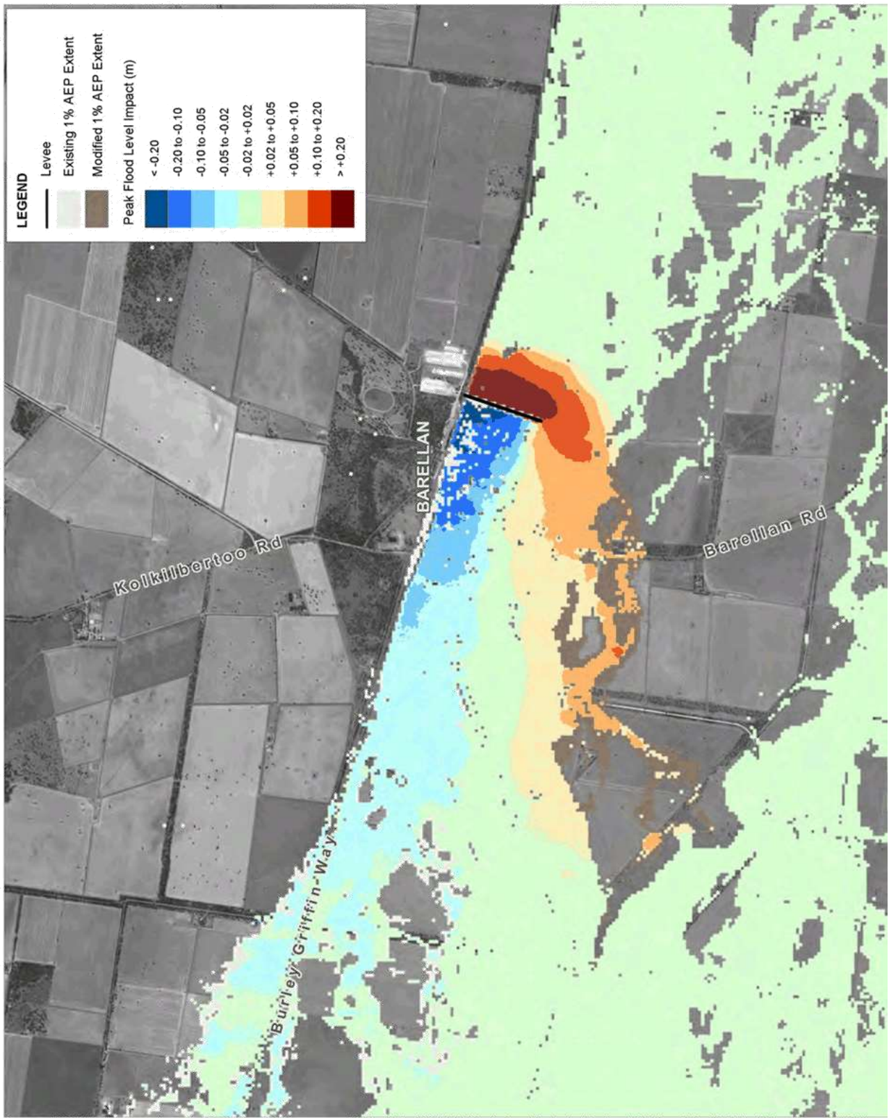
Title: Borellan FRMS&P Levee Option 1a 1% AEP Change in Peak Flood Level
