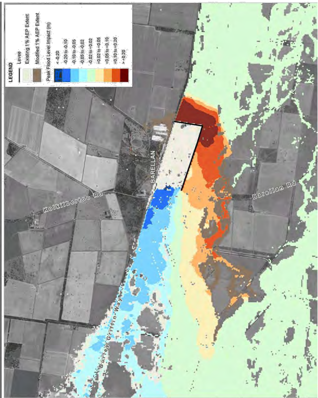
Title: Barellan FRMS&P Levee Option 1d 1% AEP Change in Peak Flood Level
